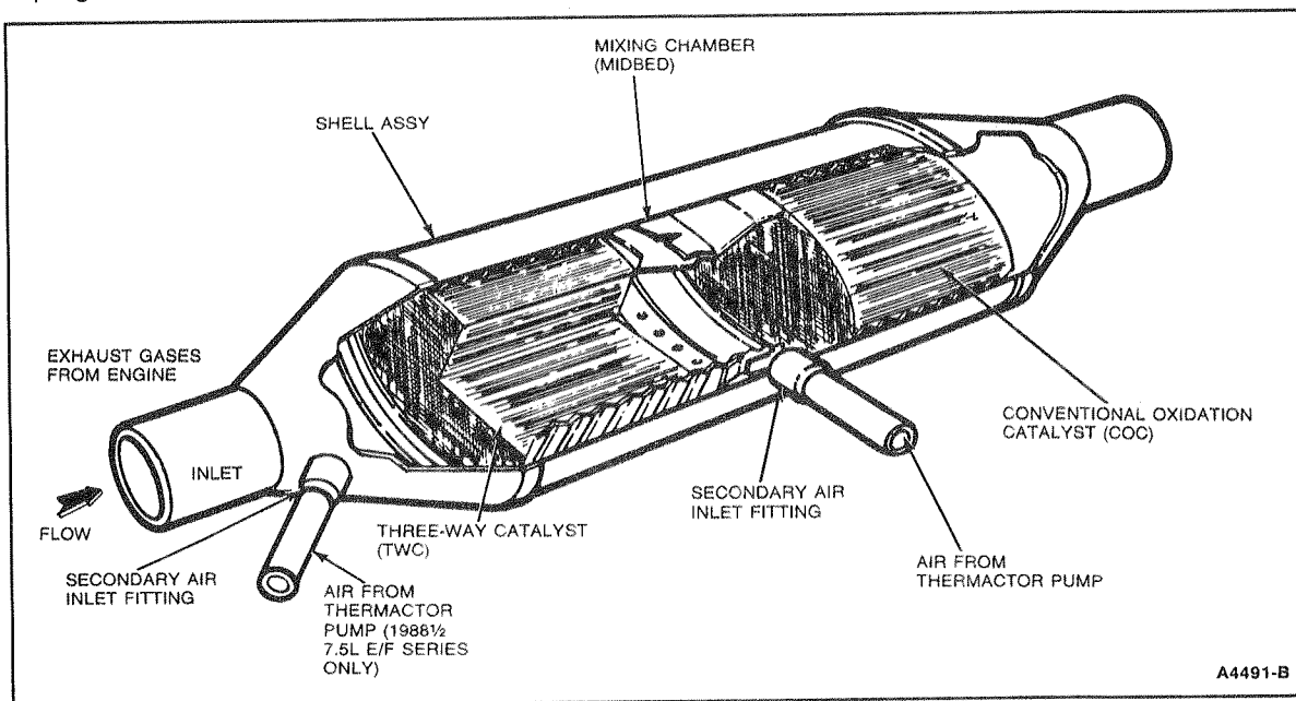
Figure 1 Dual Catalytic Converter
